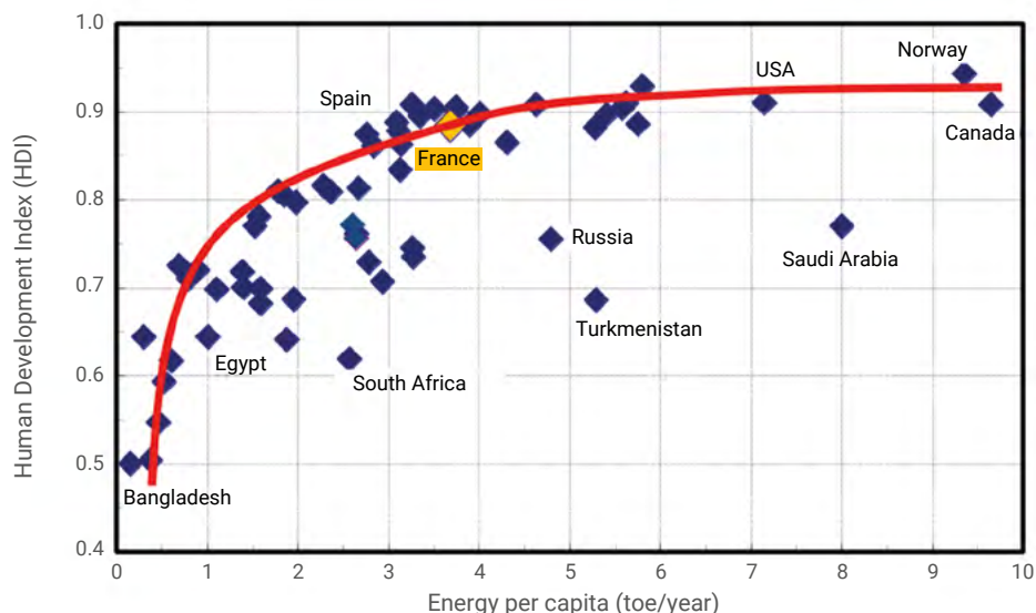
3. Human development index as a function of energy consumption, expressed in toe/year (1 toe = 11.63 MWh). Source: H. Safa [10]
