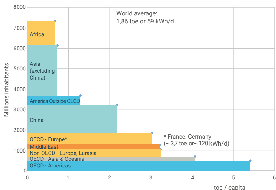
1. Regional breakdown of annual primary energy consumption per capita expressed in toe per capita (1 toe = 11.63 MWh). based on data from the International Energy Agency (IEA, www.iea.org/ ).
